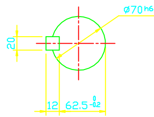
OUTPUT SHAFT
